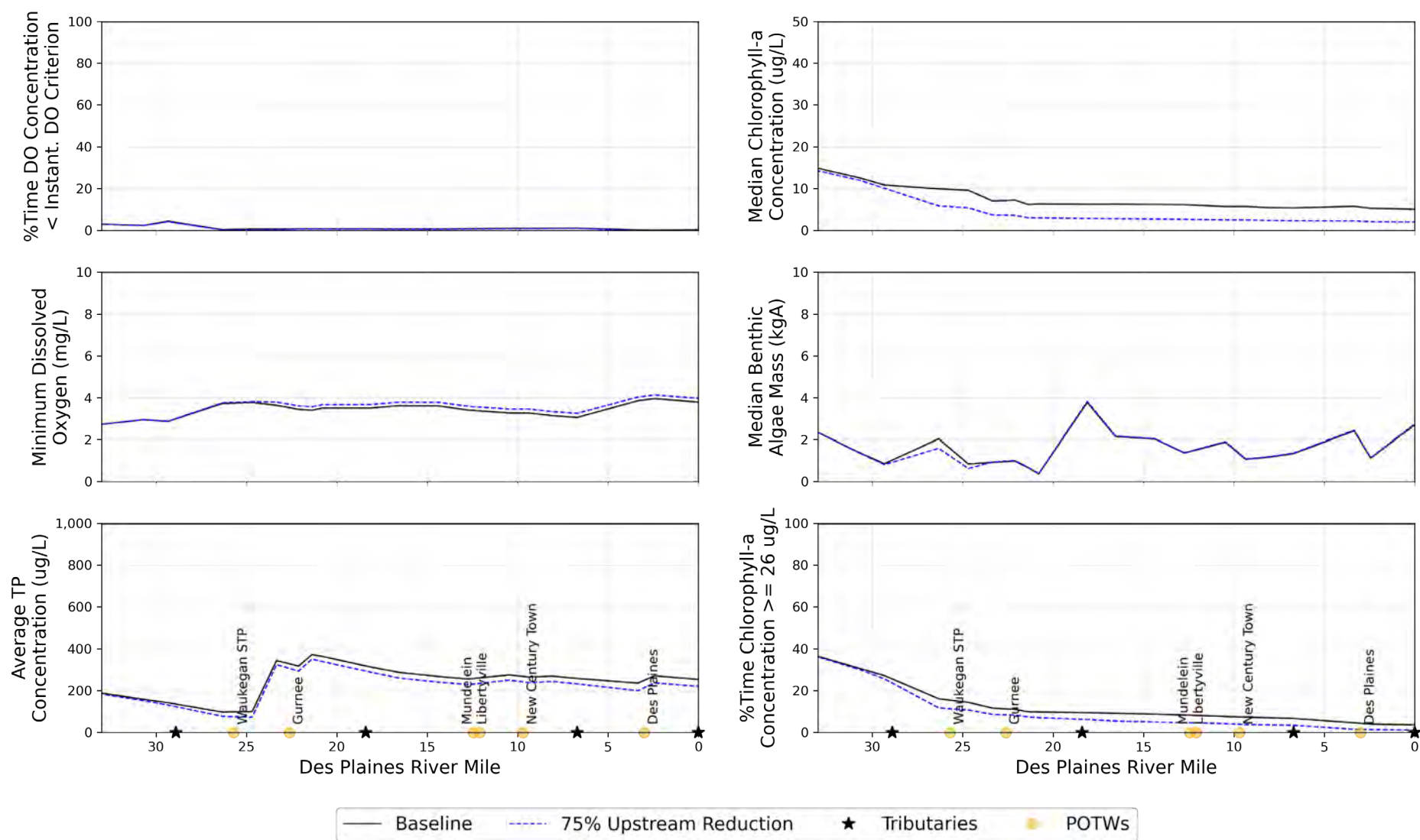
Figure 31: Upstream Load Reduction Model Results, Growing Season (May 1–October 31, 2020)
